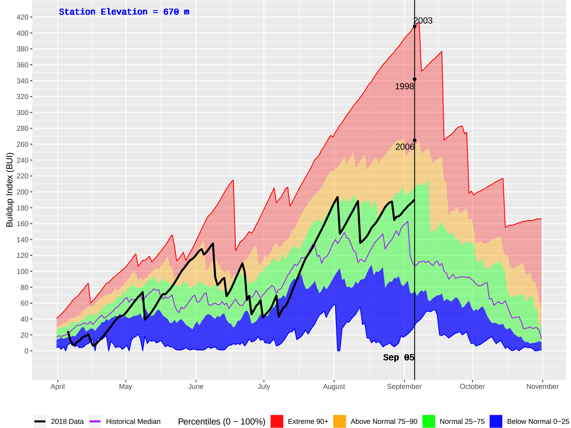
FINTRY (298) : Historical (1989–2016) and Current (2018) Daily Buildup Index (BUI)
