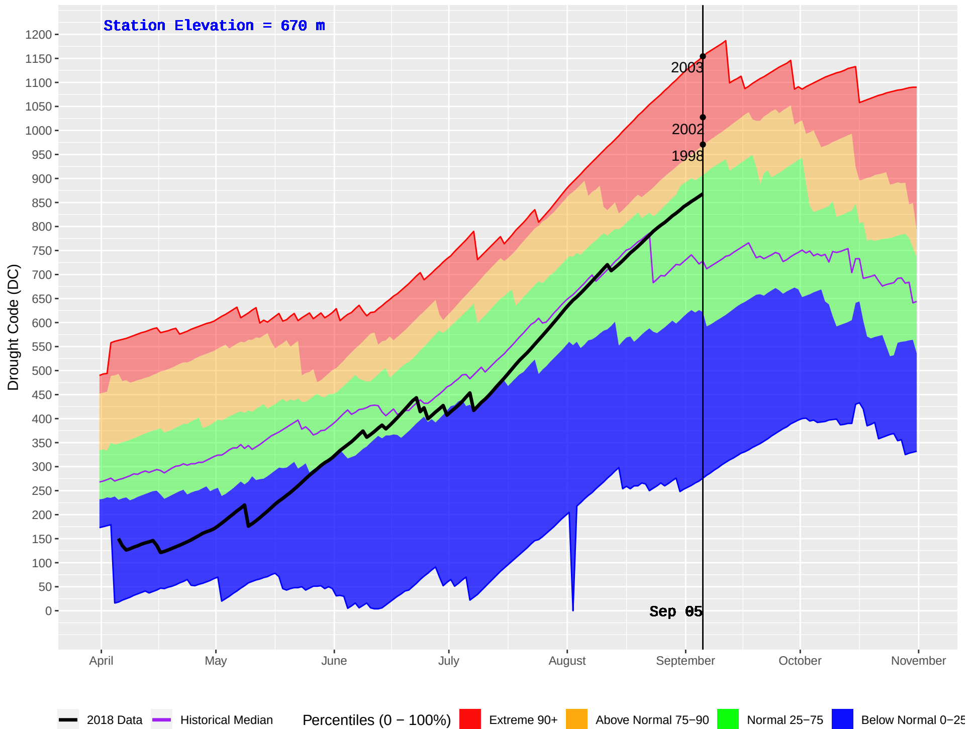
FINTRY (298) : Historical (1989–2016) and Current (2018) Daily Drought Code (DC)
