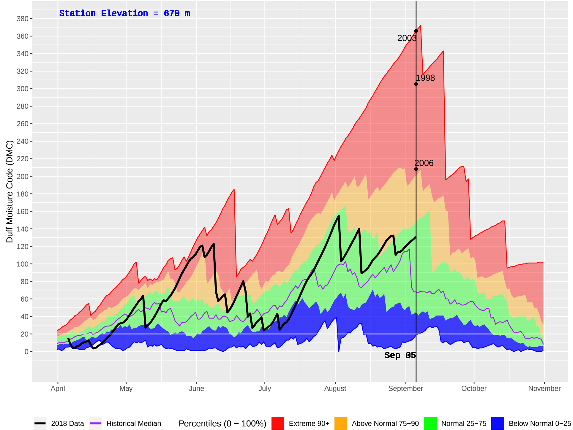
FINTRY (298) : Historical (1989–2016) and Current (2018) Daily Duff Moisture Code (DMC)
