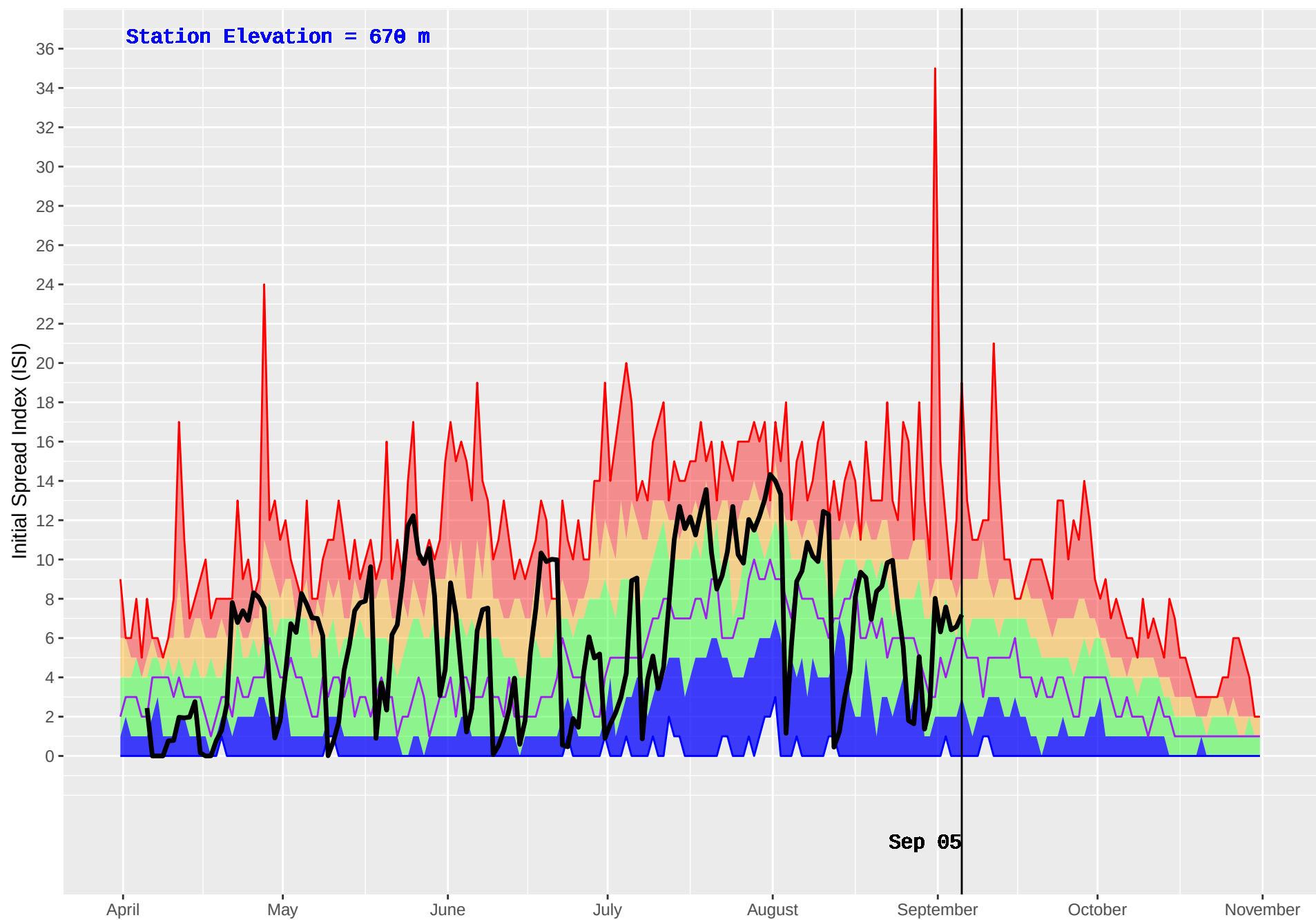
FINTRY (298) : Historical (1989–2016) and Current (2018) Daily Initial Spread Index (ISI)
