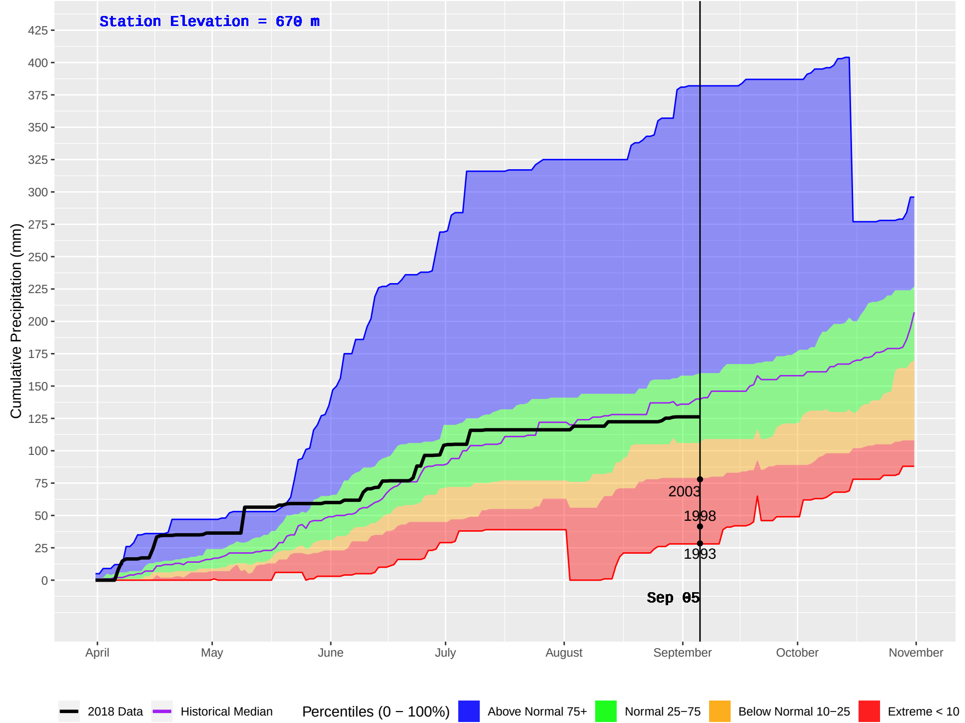
FINTRY (298) : Historical (1989–2016) and Current (2018) Daily Cumulative Precipitation
