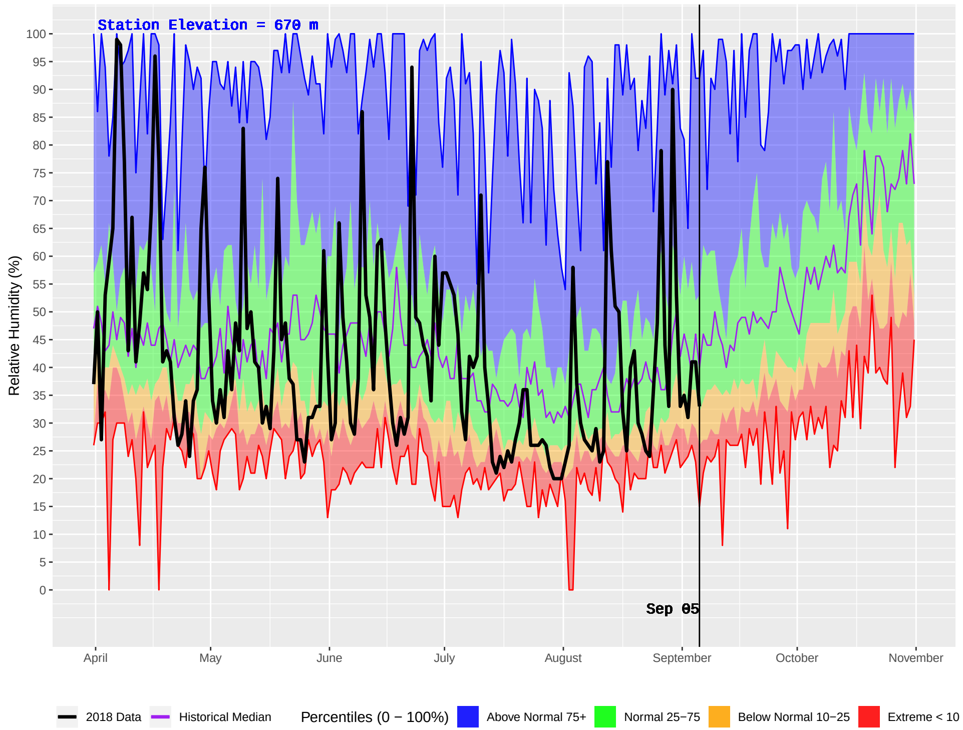
FINTRY (298) : Historical (1989–2016) and Current (2018) Daily Relative Humidity
