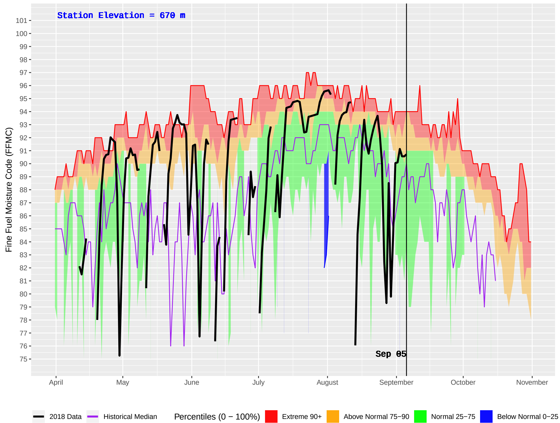
FINTRY (298) : Historical (1989–2016) and Current (2018) Daily Fine Fuel Moisture Code (FFMC)
